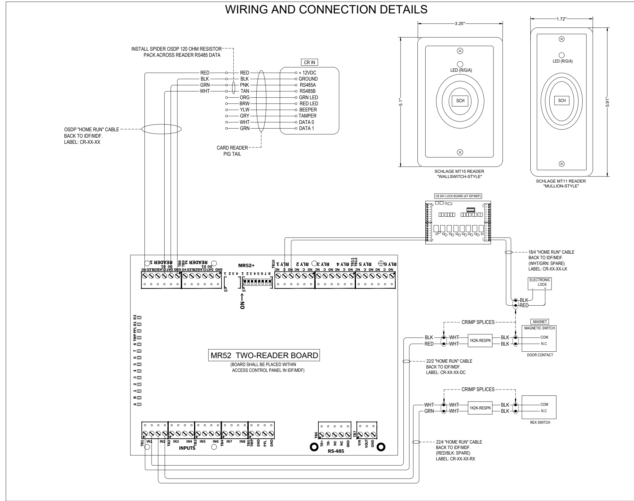
3 TYPICAL CARD READ IN / REX OUT (CR-XX-XX)
