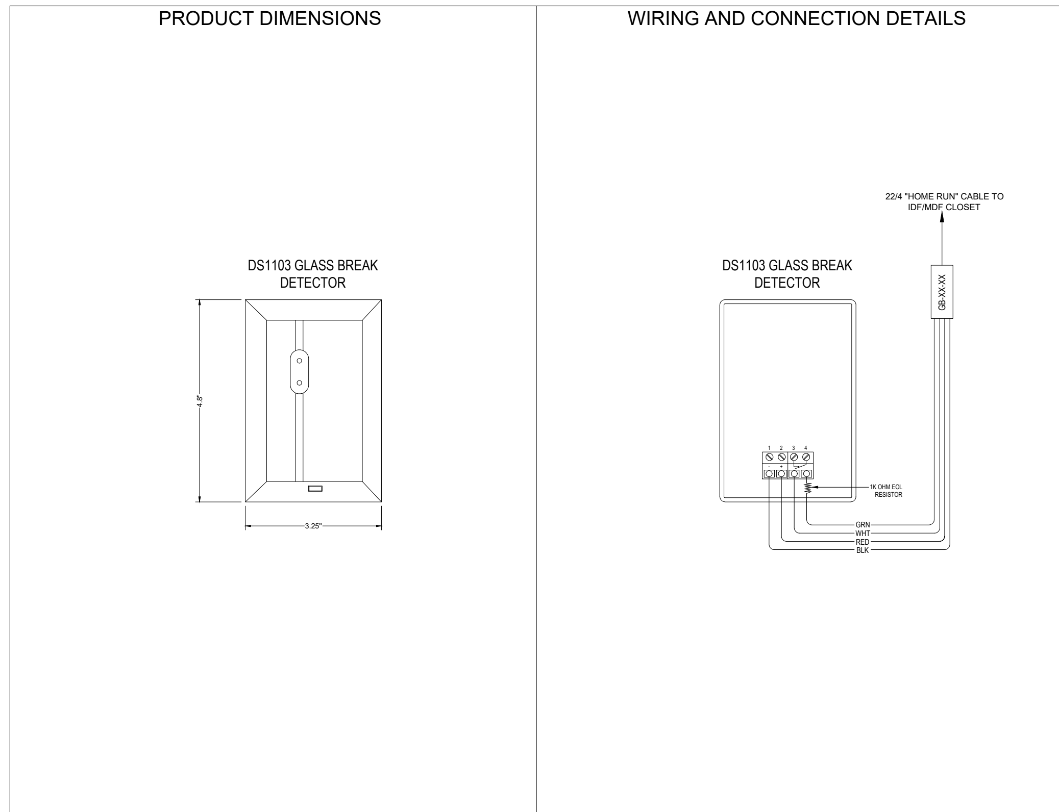
1 TYPICAL GLASS BREAK DETECTOR (GB-XX-XX) *EACH GB DIRECTLY WIRED BACK TO THE PANEL
