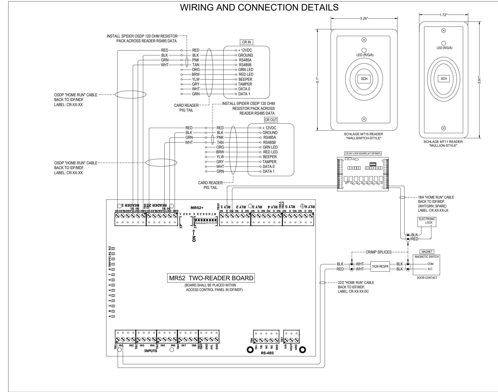
4 TYPICAL CARD READER IN / CARD READER OUT (CR-XX-XX)
