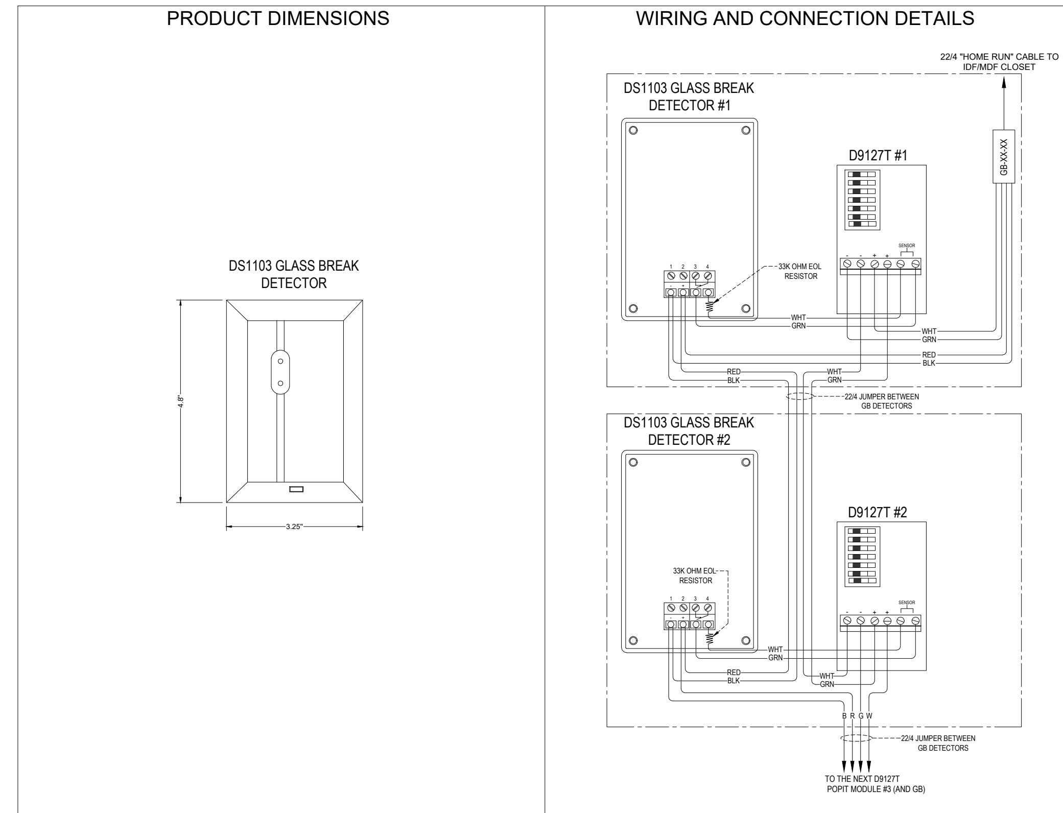
2 TYPICAL GLASS BREAK DETECTOR (GB-XX-XX) *GB'S FIELD DAISY-CHAINED USING D9127T POPIT MODULES
